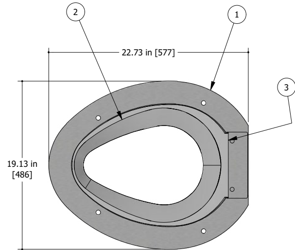
TOP VIEW (WITHOUT HINGED SEAT)
