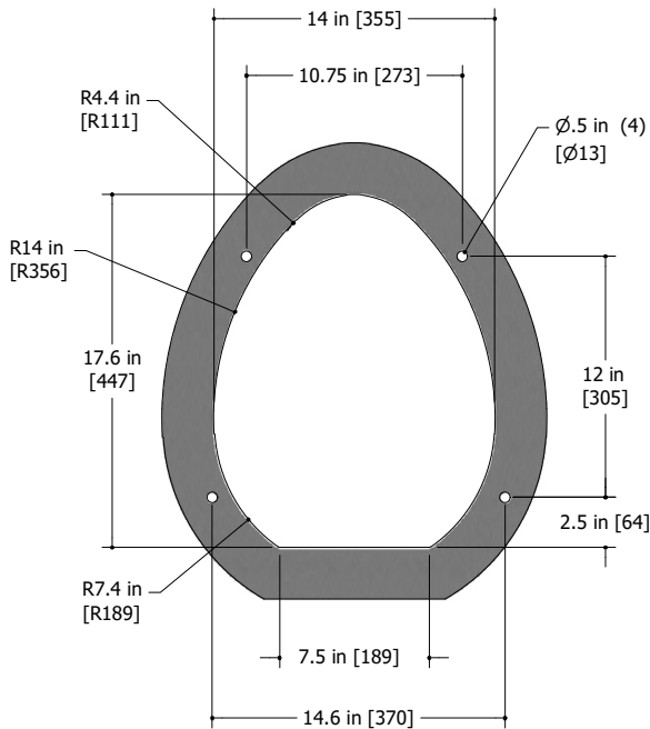
FLOOR OPENING DETAIL
