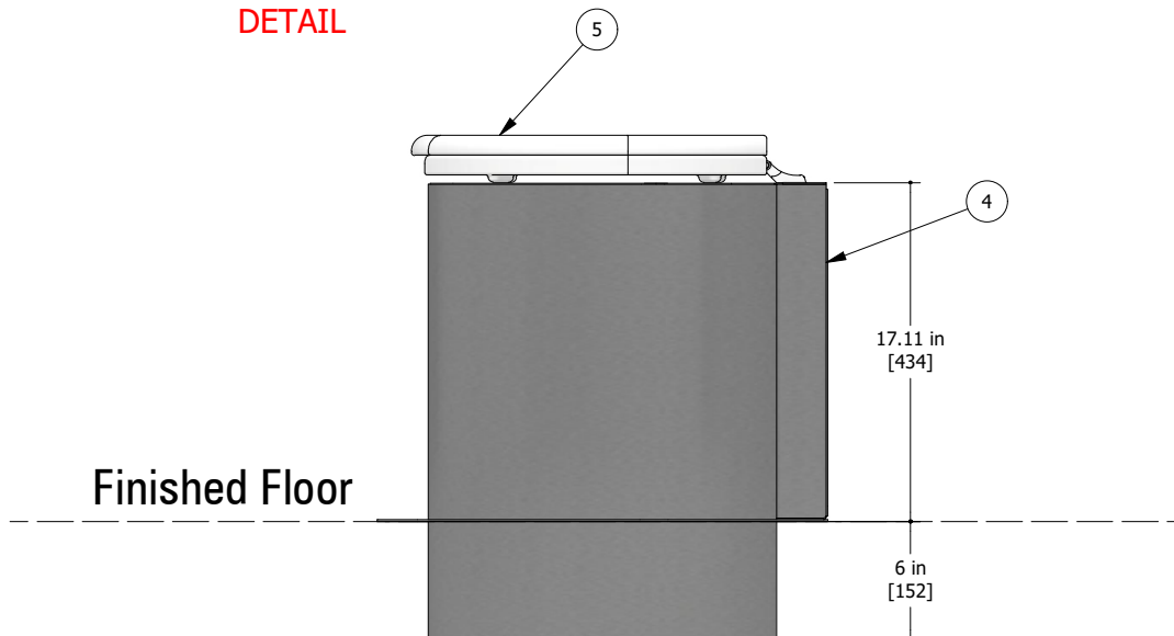
SIDE ELEVATION
