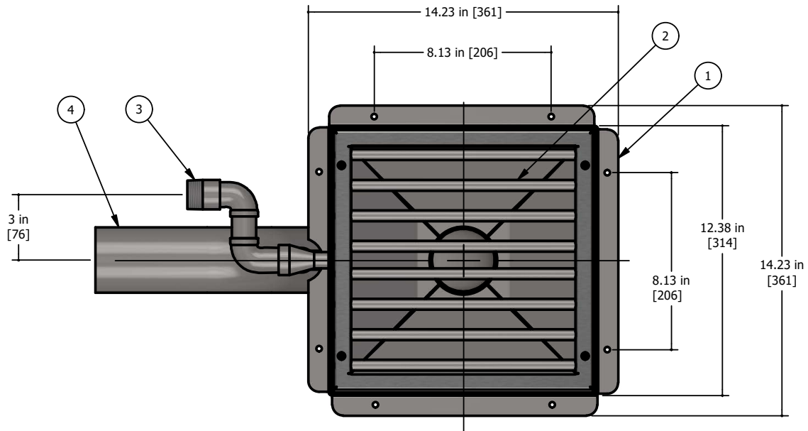
PLAN VIEW
