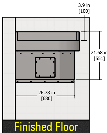
Front View of Fixture
