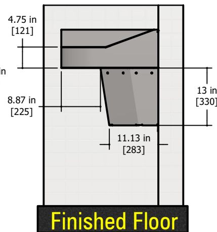
Side View of Fixture
