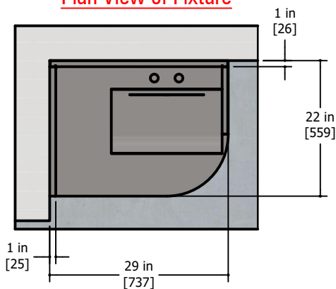
Plan View of Fixture
