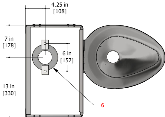
Flange Bolt Locations Plan View - Floor Outlet
